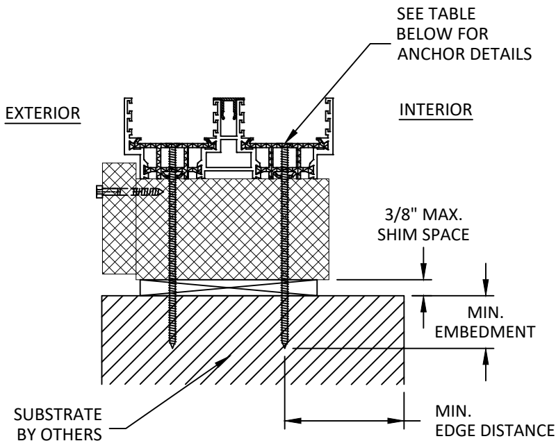
B 6 VERTICAL SECTION SILL - THROUGH FRAME
