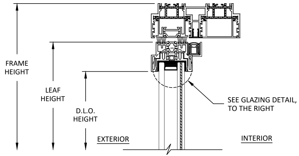
A 4 VERTICAL SECTION HEAD
