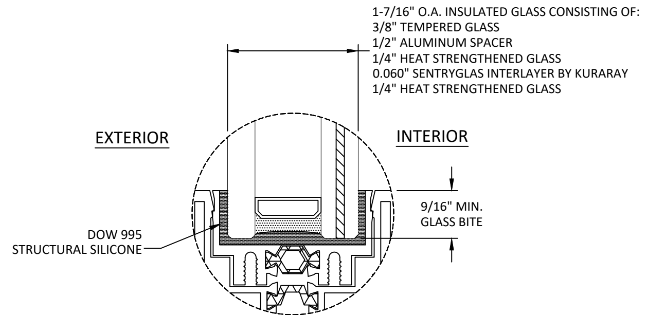
GLAZING DETAIL 1
