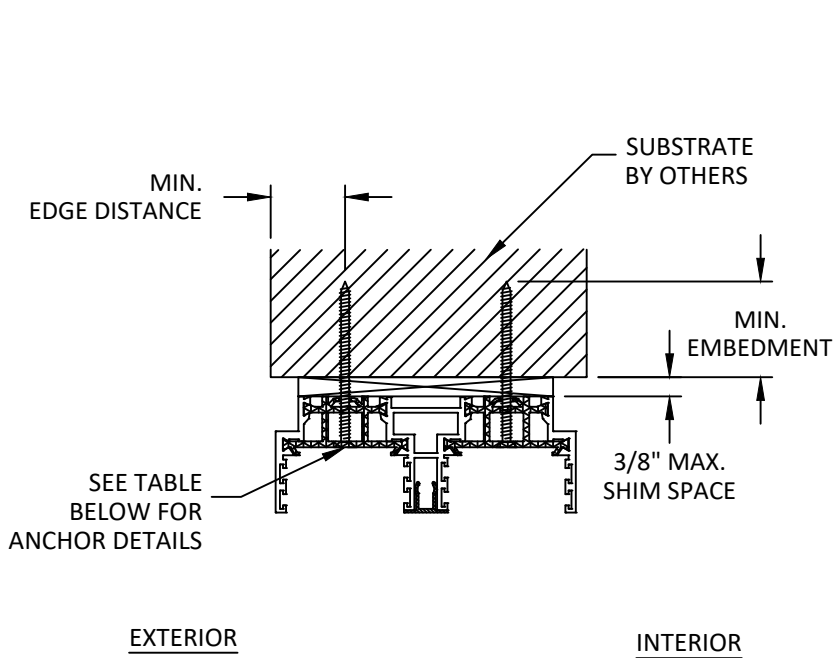
A 6 VERTICAL SECTION HEAD - THROUGH FRAME
