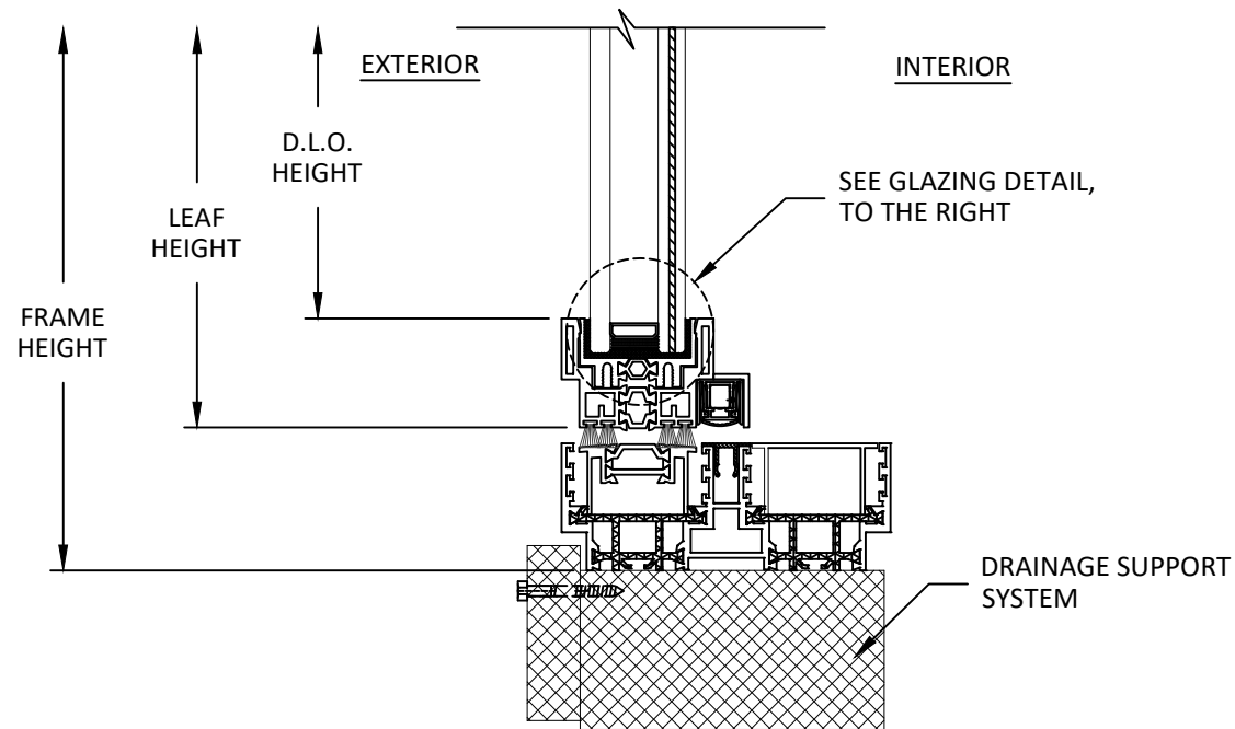
B 4 VERTICAL SECTION SILL
